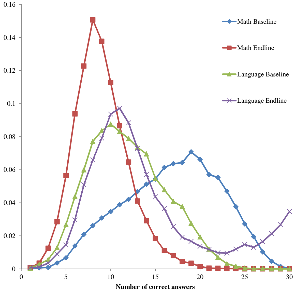
Figure 1: Probability density functions of test scores
